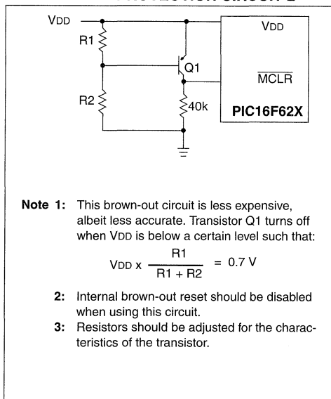
FIGURE 14-15: EXTERNAL BROWN-OUT PROTECTION CIRCUIT 2
