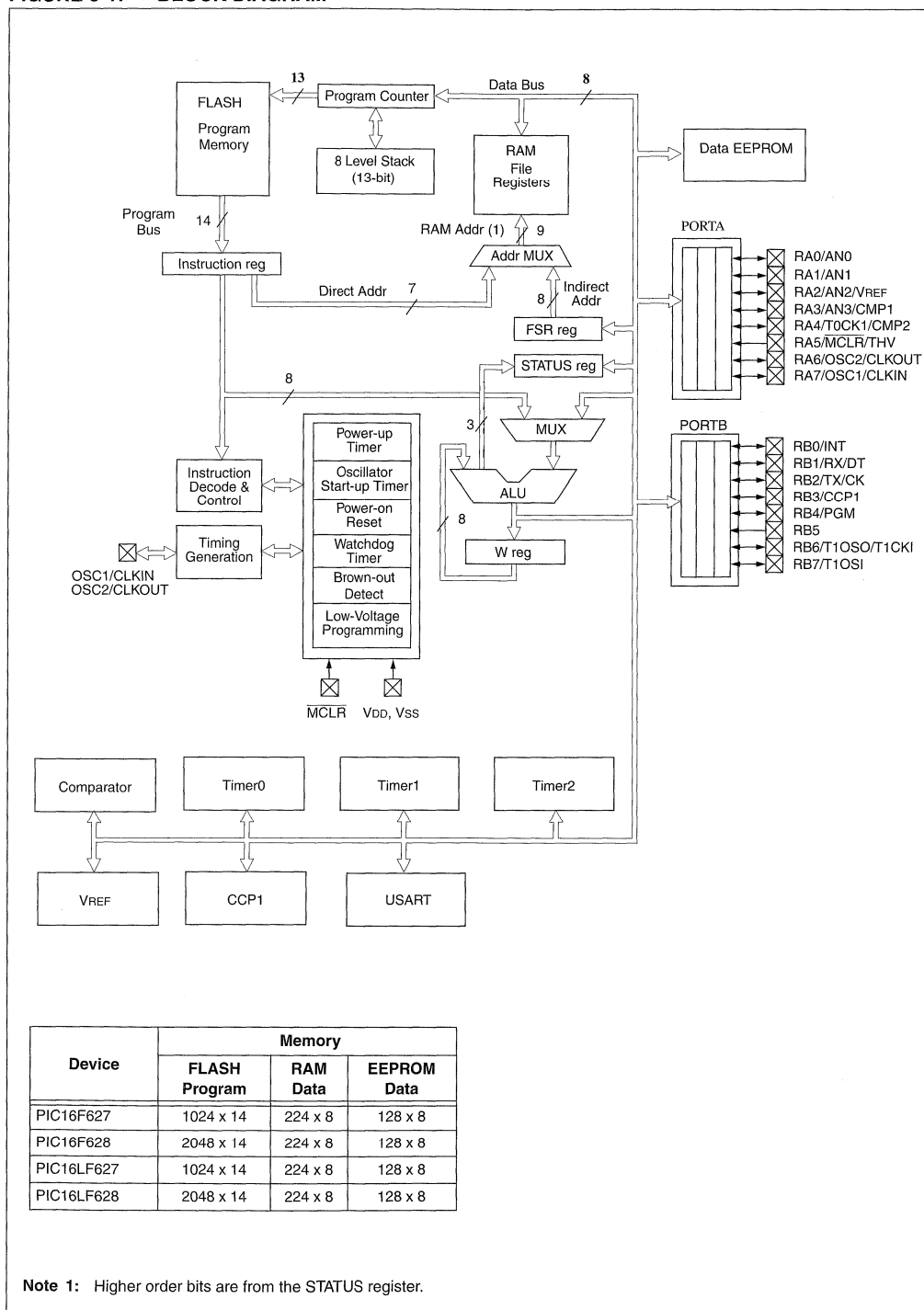
FIGURE 3-1: BLOCK DIAGRAM
