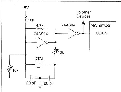
FIGURE 14-4: EXTERNAL PARALLEL RESONANT CRYSTAL OSCILLATOR CIRCUIT
