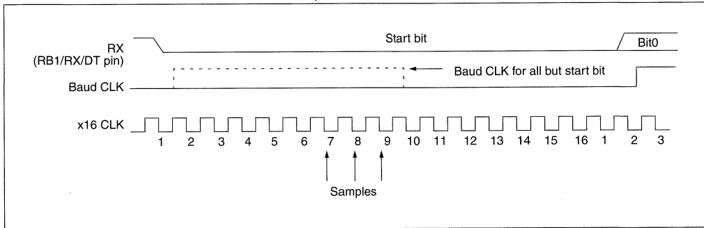
FIGURE 12-4: RX PIN SAMPLING SCHEME, BRGH = 0 OR BRGH = 1
