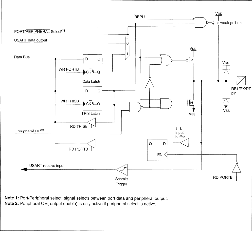
FIGURE 5-9: BLOCK DIAGRAM OF RB1/TX/DT PIN
