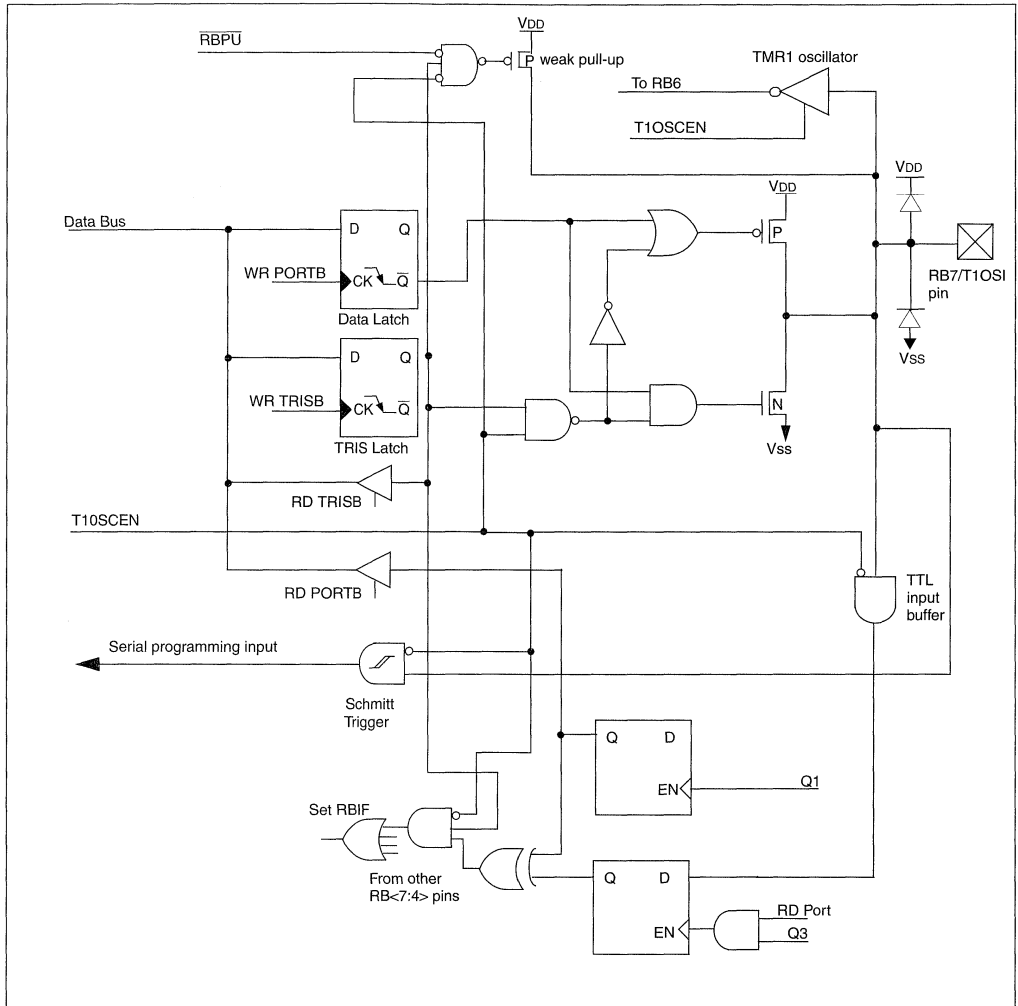
FIGURE 5-15: BLOCK DIAGRAM OF THE RB7/T1OSI PIN
