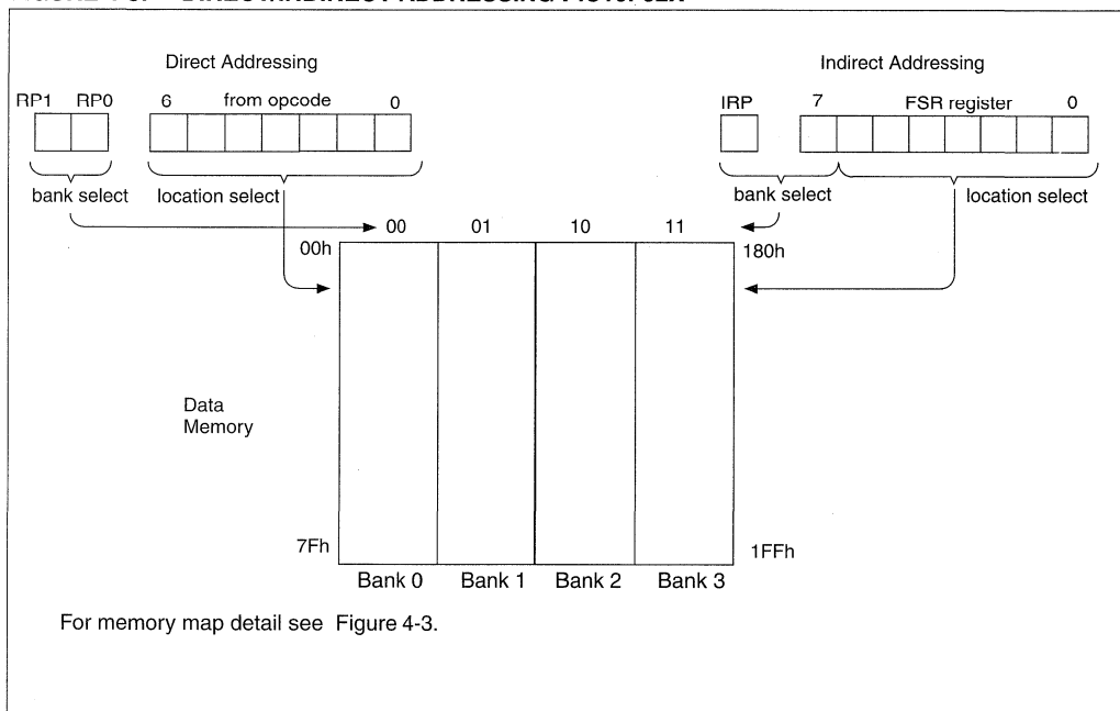
FIGURE 4-8: DIRECT/INDIRECT ADDRESSING PIC16F62X
