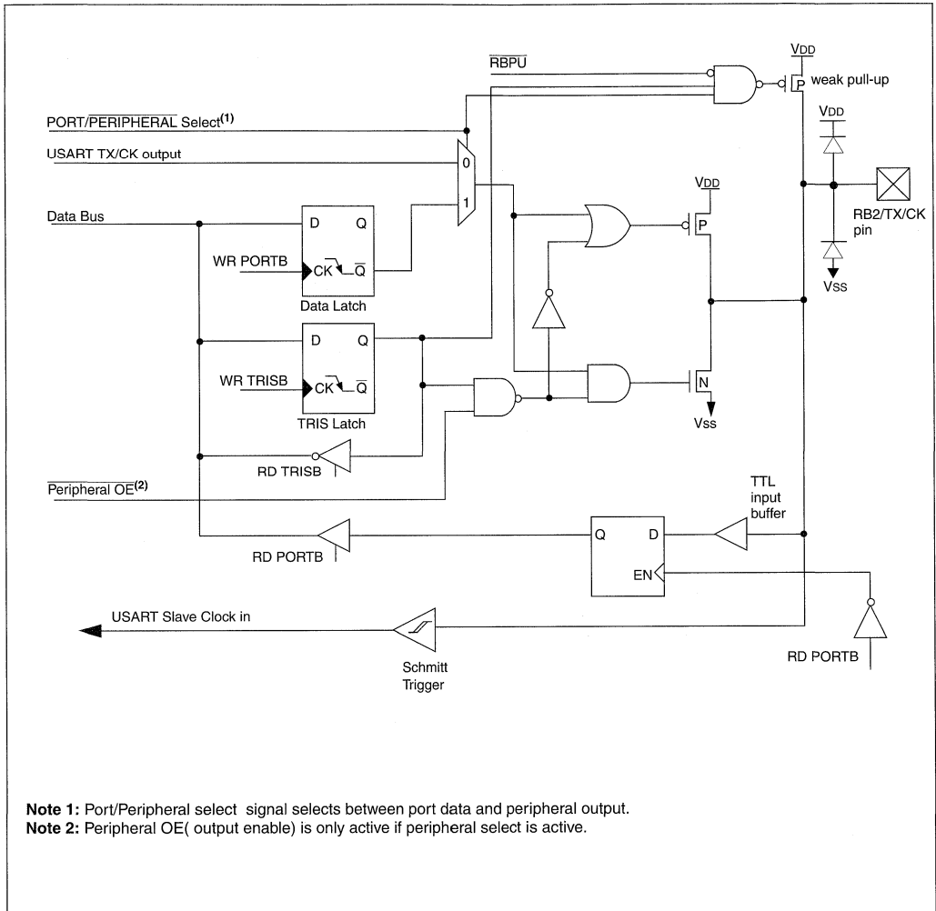
FIGURE 5-10: BLOCK DIAGRAM OF RB2/TX/CK PIN
