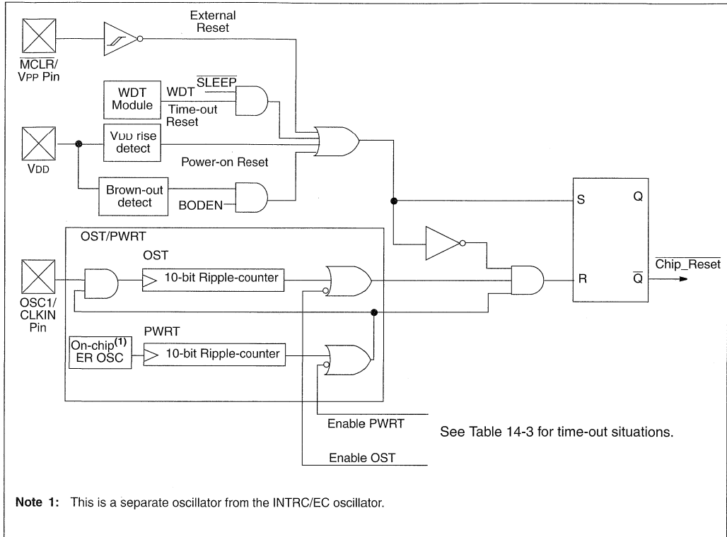
FIGURE 14-8: SIMPLIFIED BLOCK DIAGRAM OF ON-CHIP RESET CIRCUIT
