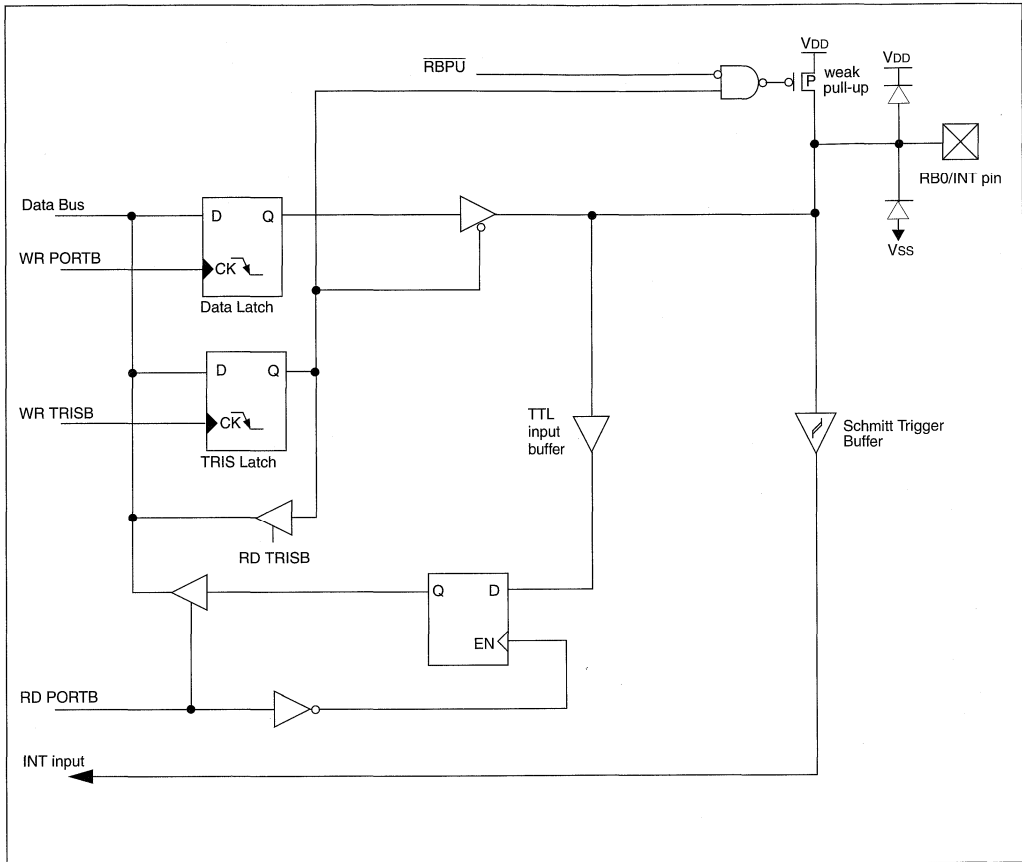
FIGURE 5-8: BLOCK DIAGRAM OF RB0/INT PIN
