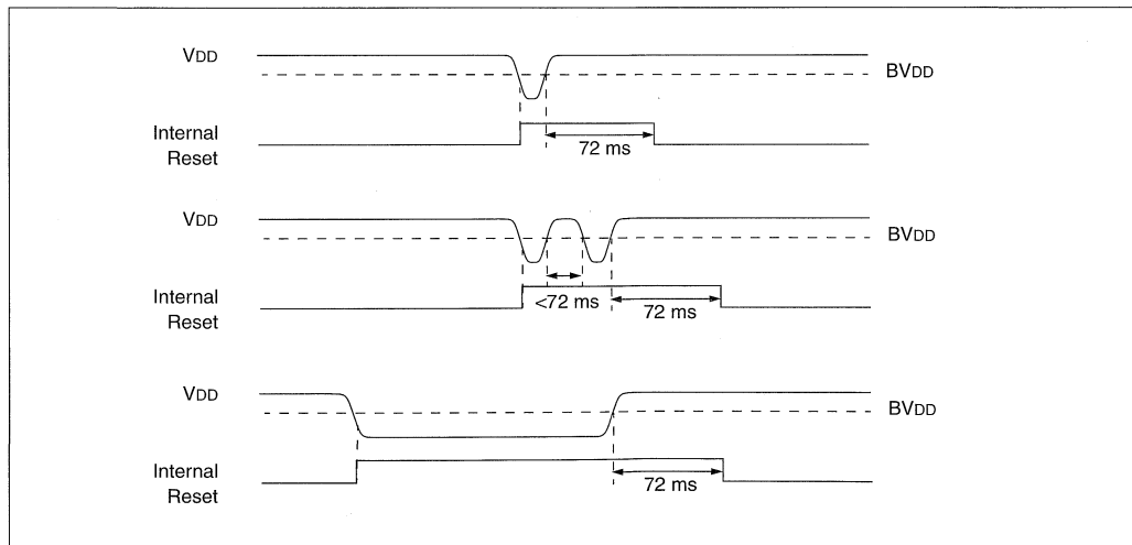
FIGURE 14-9: BROWN-OUT SITUATIONS
