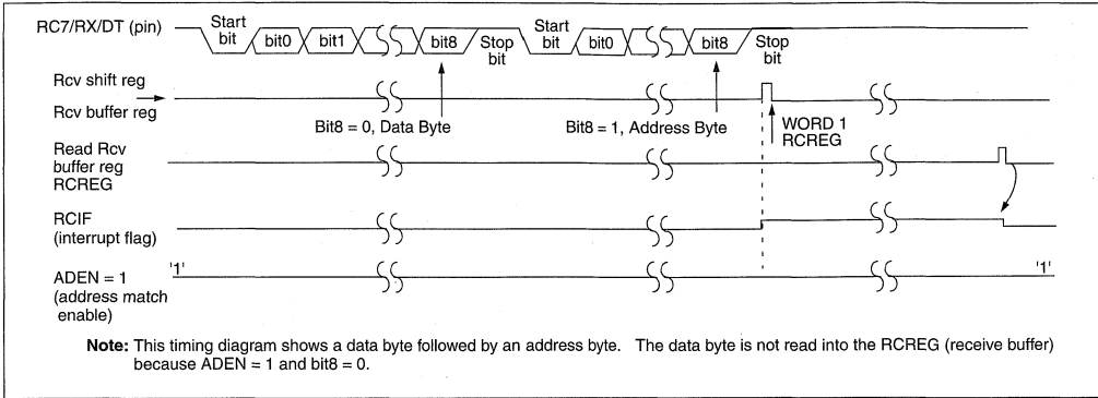
FIGURE 12-10: ASYNCHRONOUS RECEPTION WITH ADDRESS BYTE FIRST
