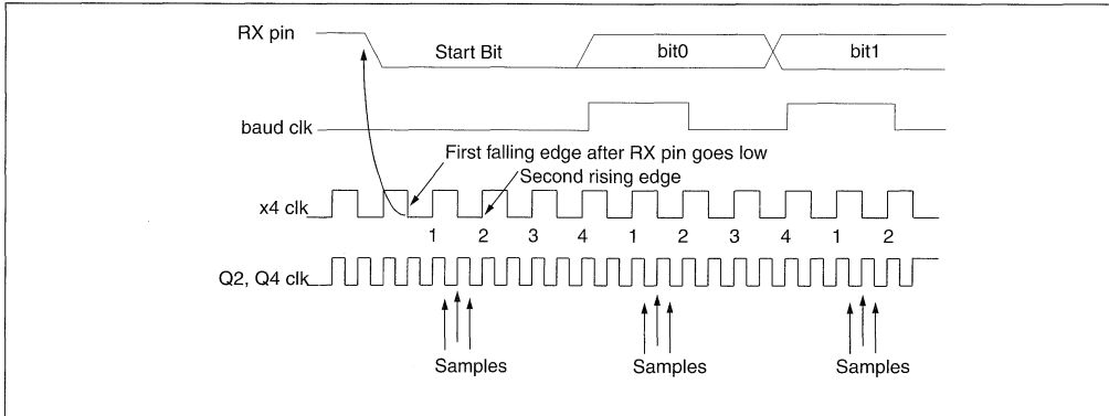
FIGURE 12-2: RX PIN SAMPLING SCHEME, BRGH = 1
