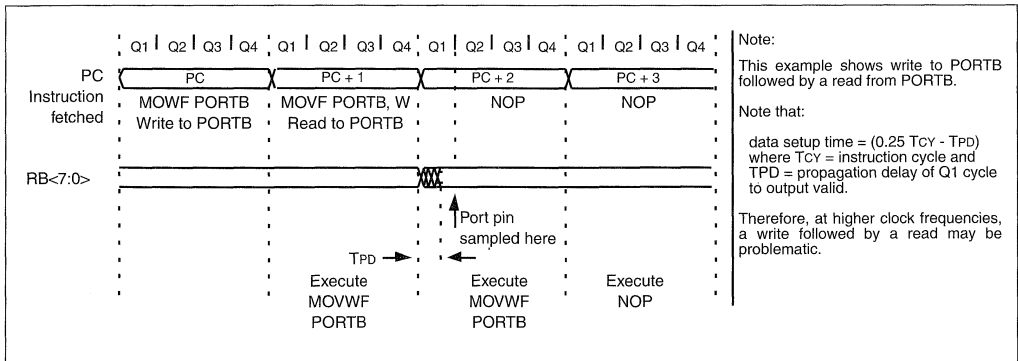
FIGURE 5-16: SUCCESSIVE I/O OPERATION
