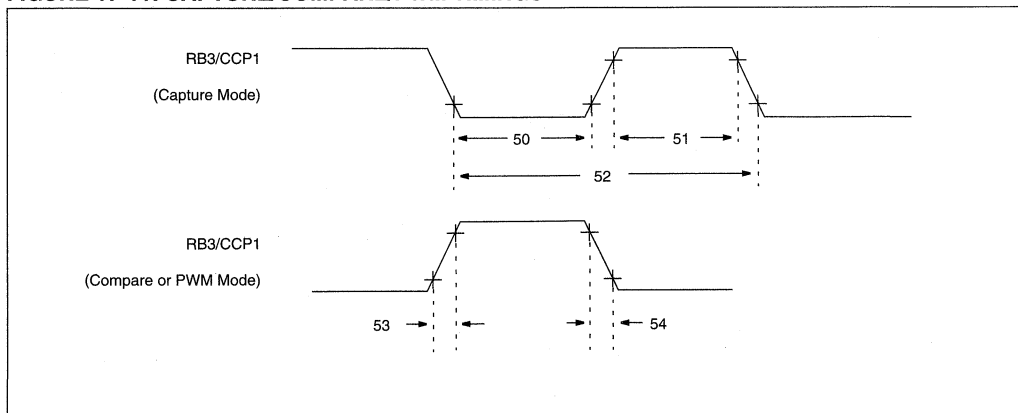
FIGURE 17-11: CAPTURE/COMPARE/PWM TIMINGS
