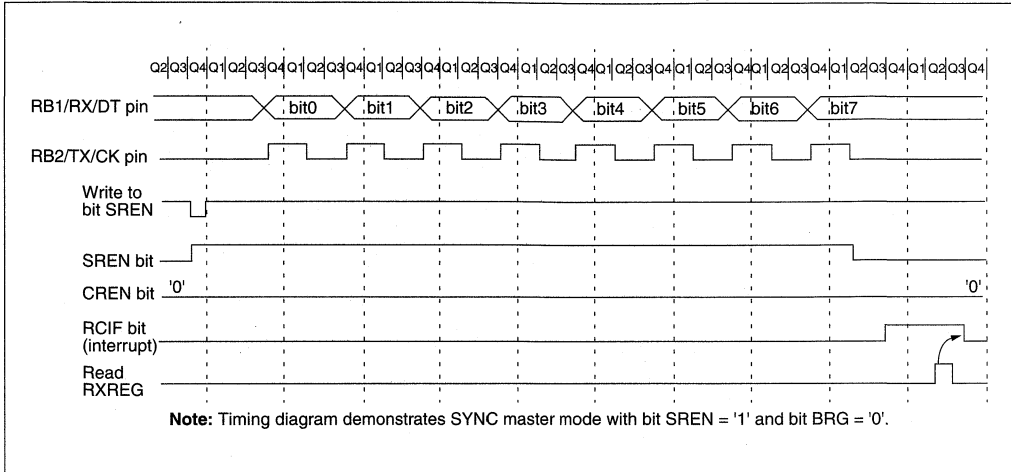
FIGURE 12-14: SYNCHRONOUS RECEPTION (MASTER MODE, SREN)
