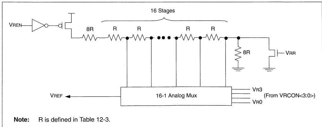
FIGURE 11-2: VOLTAGE REFERENCE BLOCK DIAGRAM
