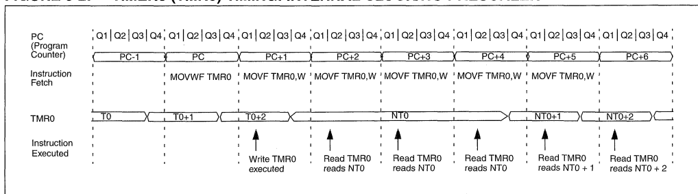
FIGURE 6-2: TIMER0 (TMR0) TIMING: INTERNAL CLOCK/NO PRESCALER
