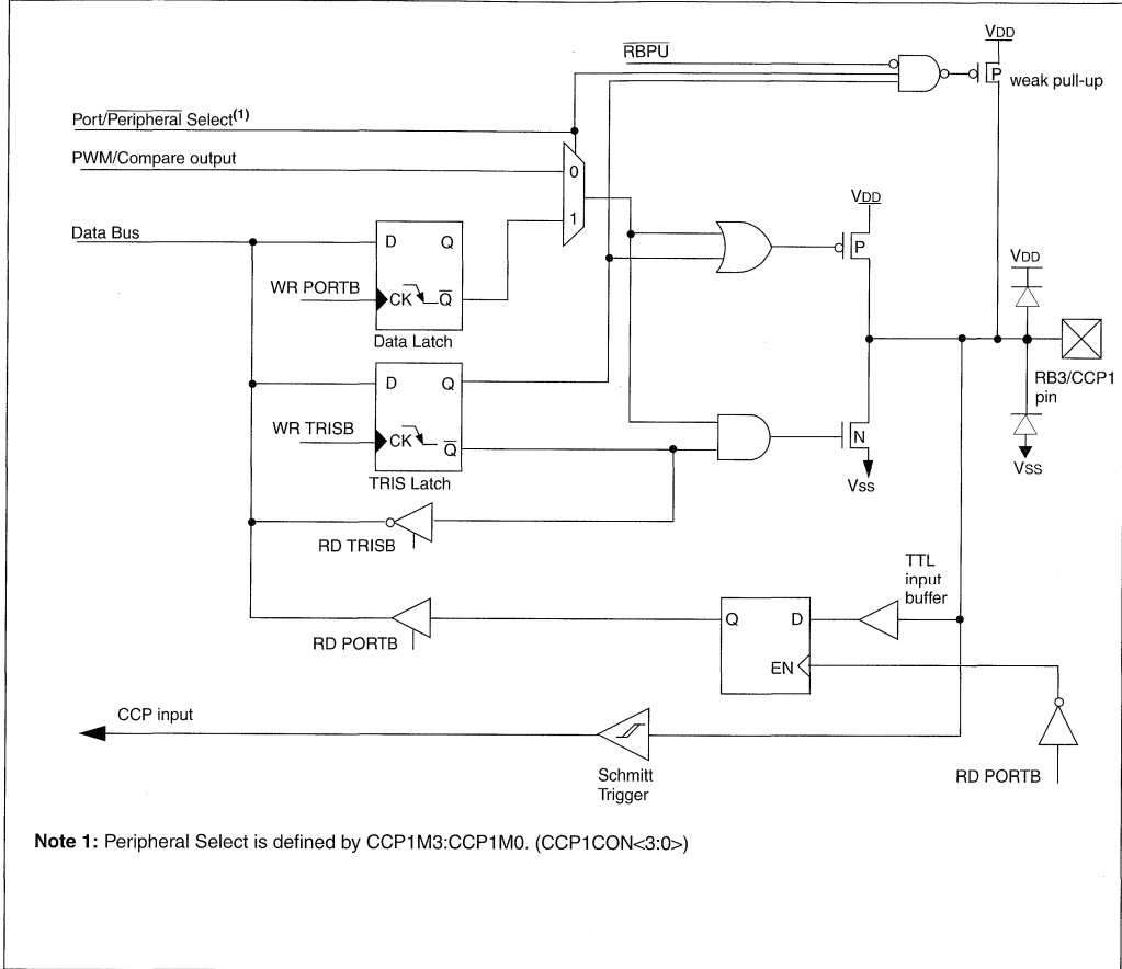
FIGURE 5-11: BLOCK DIAGRAM OF THE RB3/CCP1 PIN
