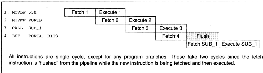
EXAMPLE 3-1: INSTRUCTION PIPELINE FLOW
