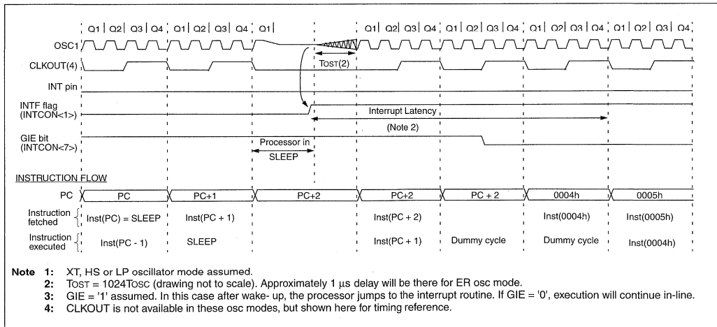
FIGURE 14-19: WAKE-UP FROM SLEEP THROUGH INTERRUPT
