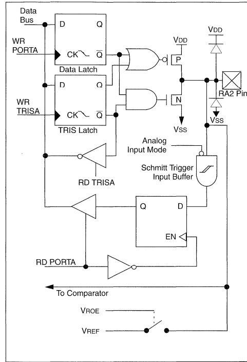
FIGURE 5-2: BLOCK DIAGRAM OF RA2/VREF PIN
