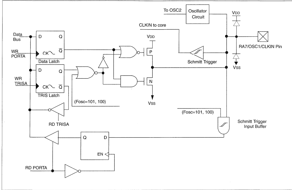
FIGURE 5-7: BLOCK DIAGRAM OF RA7/OSC1/CLKIN PIN
