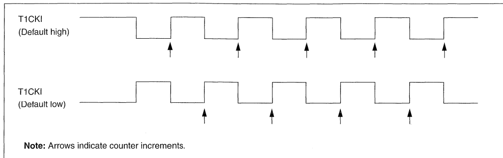
FIGURE 7-2: TIMER1 INCREMENTING EDGE
