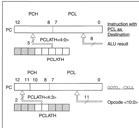
FIGURE 4-7: LOADING OF PC IN DIFFERENT SITUATIONS
