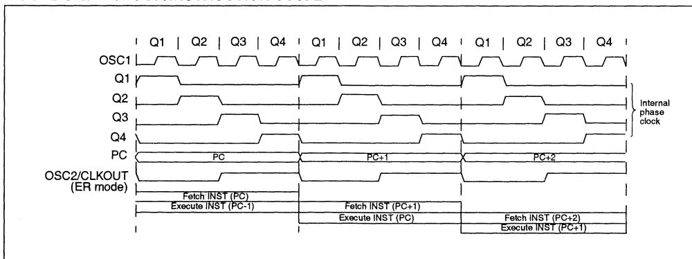
EXAMPLE 3-1: INSTRUCTION PIPELINE FLOW
