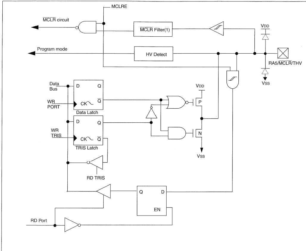
FIGURE 5-5: BLOCK DIAGRAM OF THE RA5/MCLR/THV PIN
