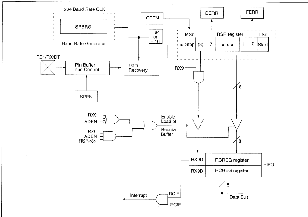
FIGURE 12-8: USART RECEIVE BLOCK DIAGRAM
