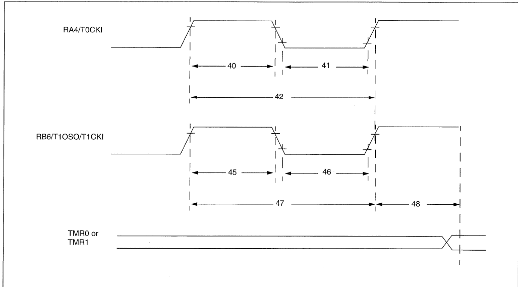
FIGURE 17-10: TIMER0 AND TIMER1 EXTERNAL CLOCK TIMINGS
