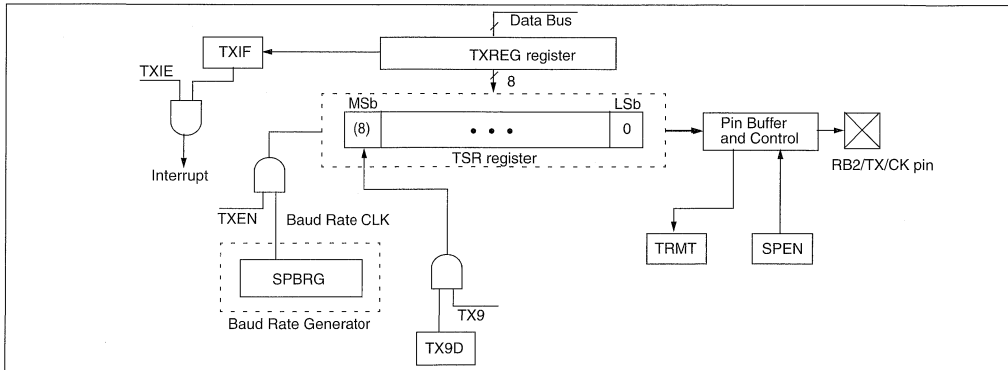
FIGURE 12-5: USART TRANSMIT BLOCK DIAGRAM
