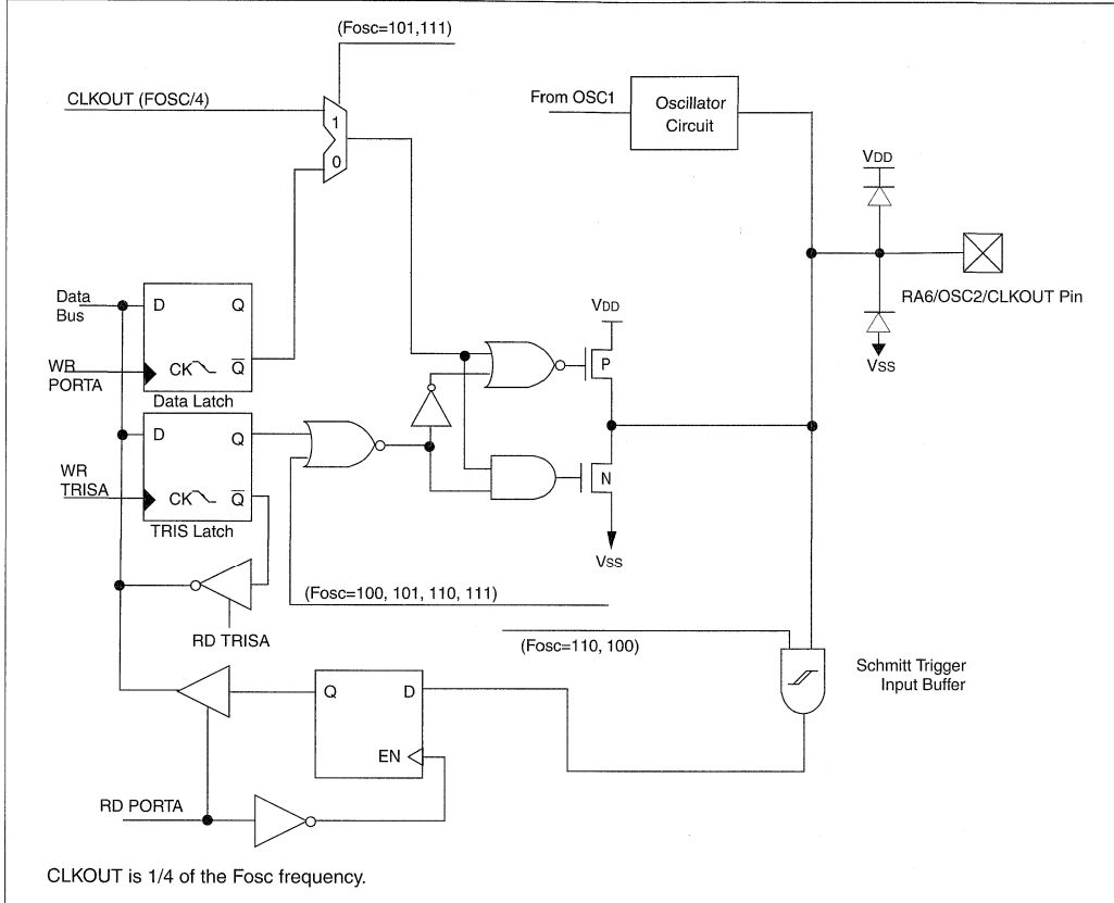
FIGURE 5-6: BLOCK DIAGRAM OF RA6/OSC2/CLKOUT PIN
