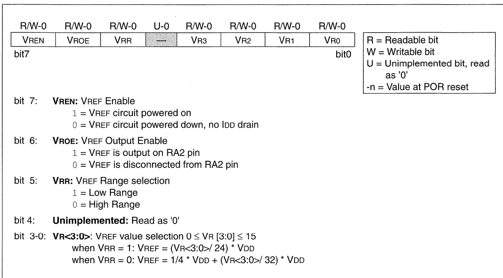
FIGURE 11-1: VRCON REGISTER (ADDRESS 9Fh)
