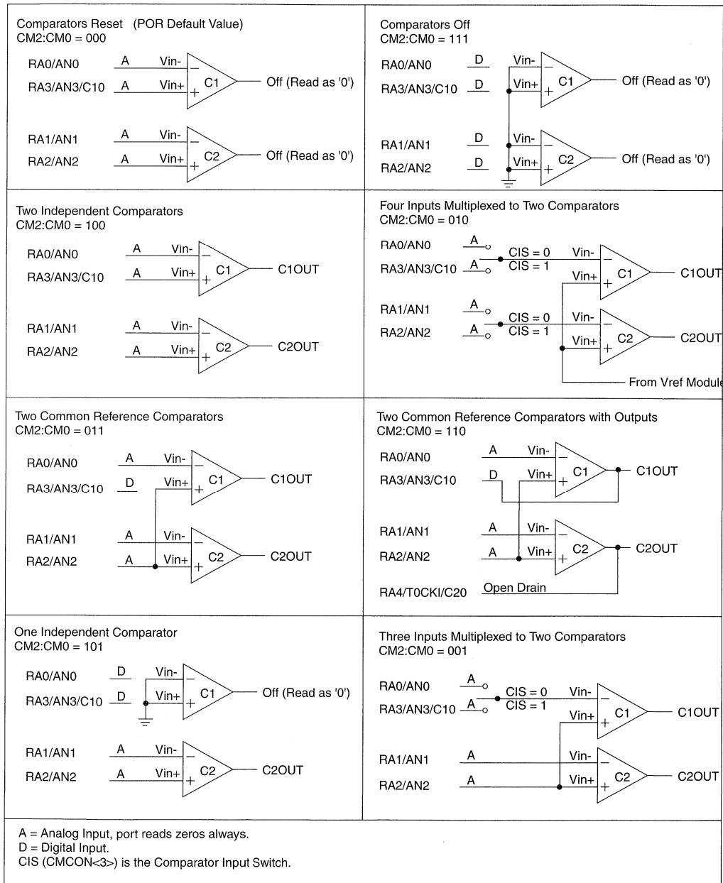
FIGURE 9-1: COMPARATOR I/O OPERATING MODES
