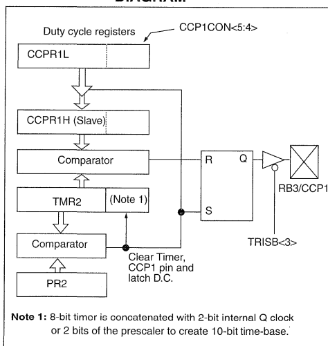
FIGURE 10-3: SIMPLIFIED PWM BLOCK DIAGRAM
