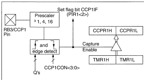
FIGURE 10-1: CAPTURE MODE OPERATION BLOCK DIAGRAM
