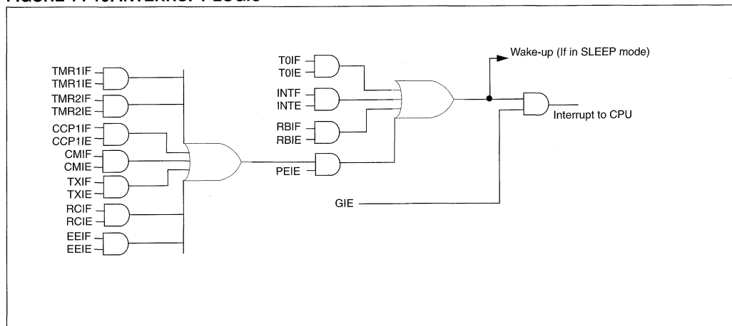
FIGURE 14-16: INTERRUPT LOGIC
