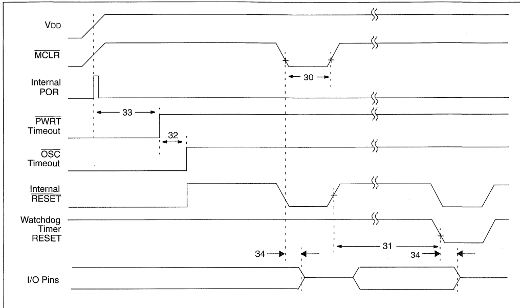
FIGURE 17-9: BROWN-OUT DETECT TIMING
