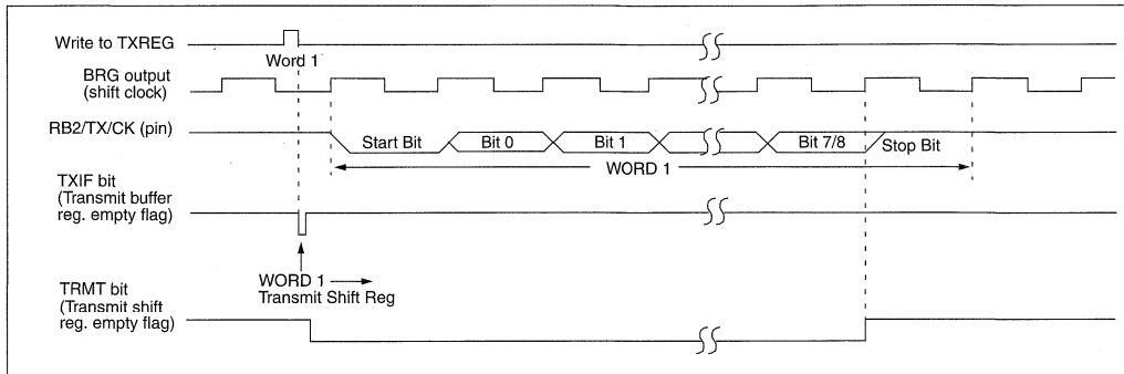
FIGURE 12-7: ASYNCHRONOUS MASTER TRANSMISSION (BACK TO BACK)
