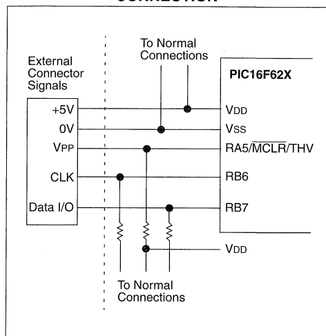
FIGURE 14-20: TYPICAL IN-CIRCUIT SERIAL PROGRAMMING CONNECTION
