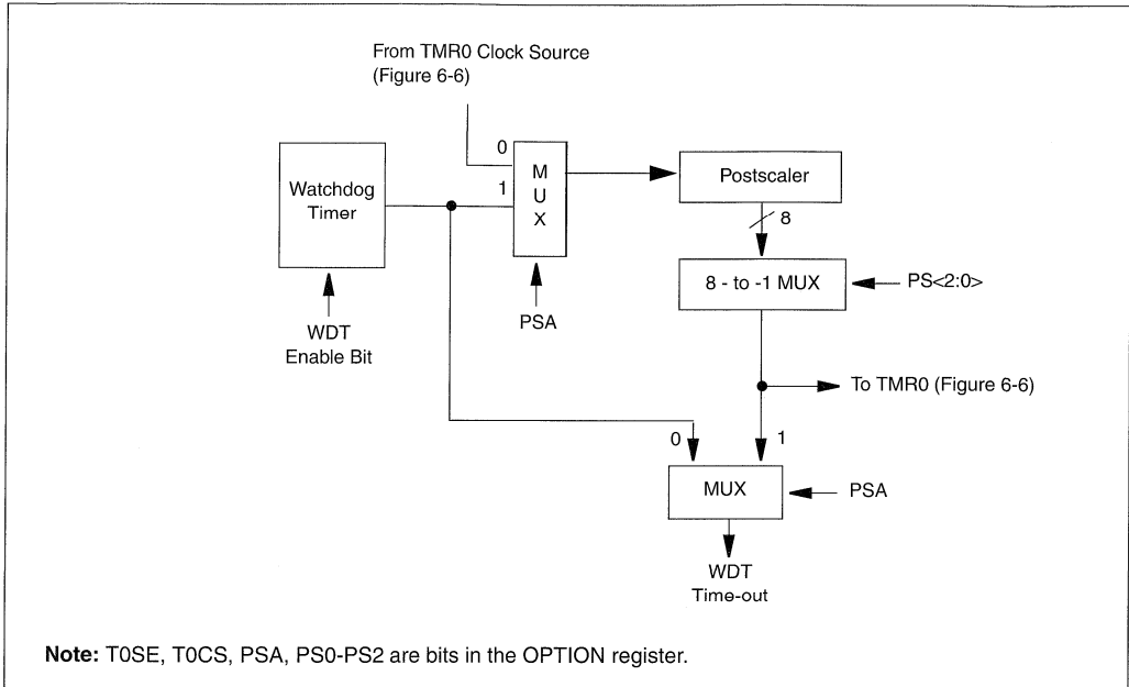
FIGURE 14-18: WATCHDOG TIMER BLOCK DIAGRAM
