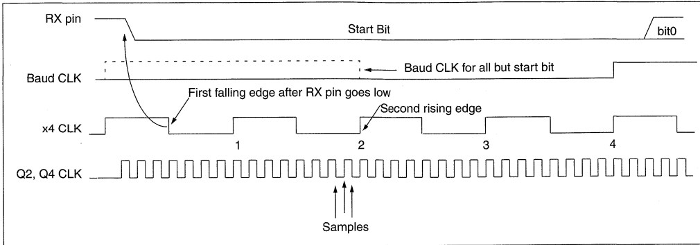
FIGURE 12-4: RX PIN SAMPLING SCHEME, BRGH = 0 OR BRGH = 1
