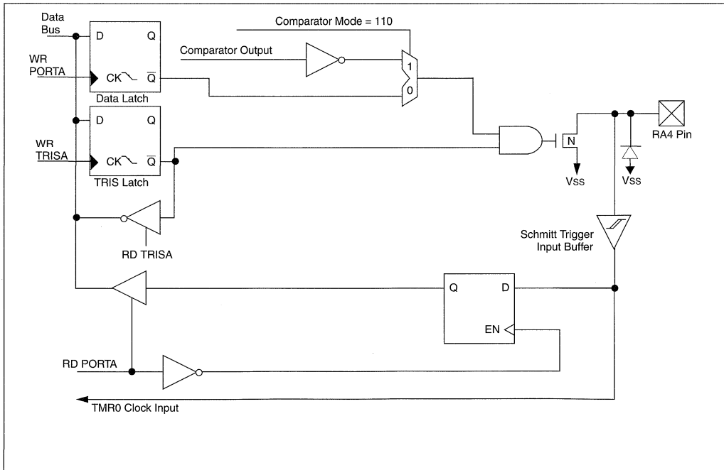
FIGURE 5-4: BLOCK DIAGRAM OF RA4/T0CKI PIN
