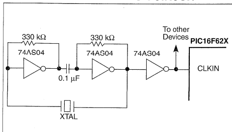
FIGURE 14-5: EXTERNAL SERIES RESONANT CRYSTAL OSCILLATOR CIRCUIT
