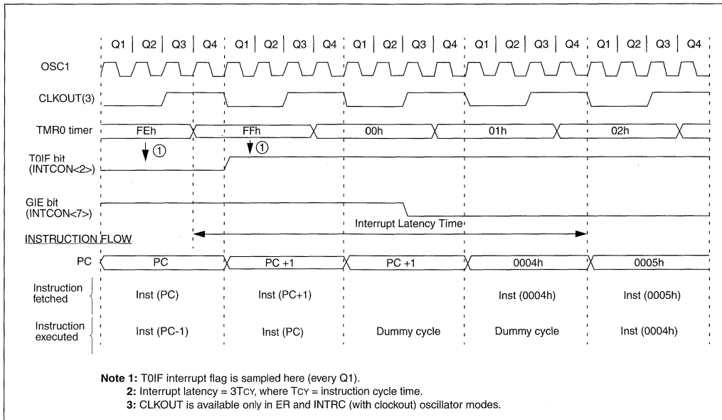
FIGURE 6-4: TIMER0 INTERRUPT TIMING
