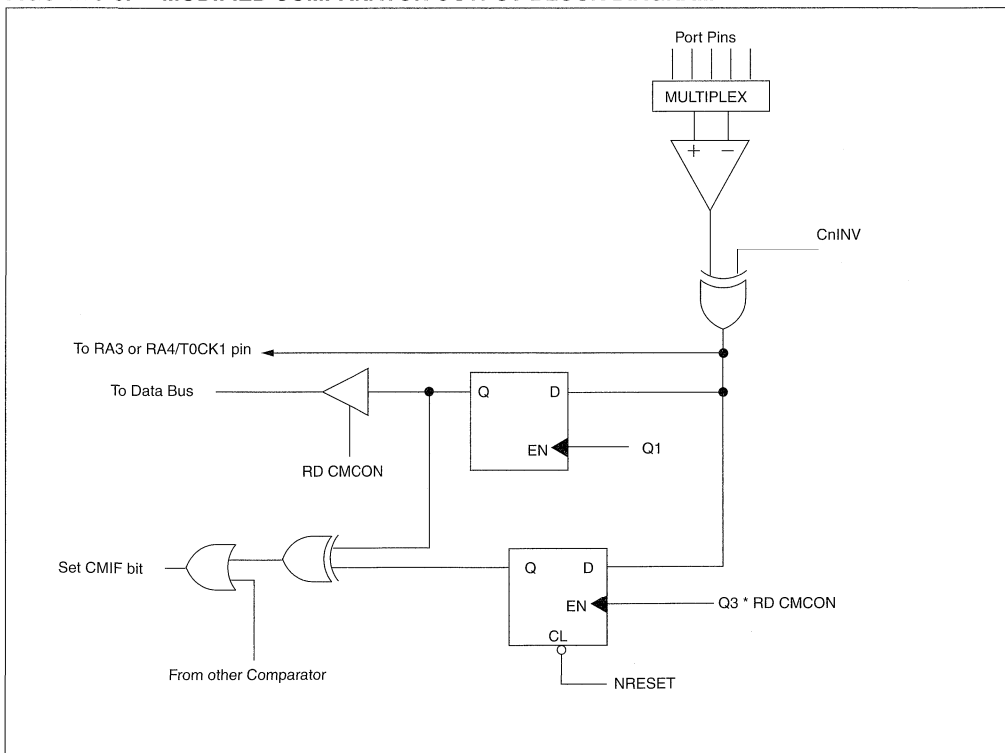
FIGURE 9-3: MODIFIED COMPARATOR OUTPUT BLOCK DIAGRAM
