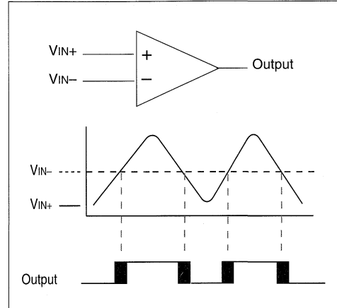
FIGURE 9-2: SINGLE COMPARATOR
