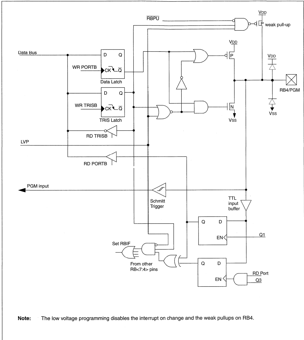
FIGURE 5-12: BLOCK DIAGRAM OF RB4/PGM PIN
