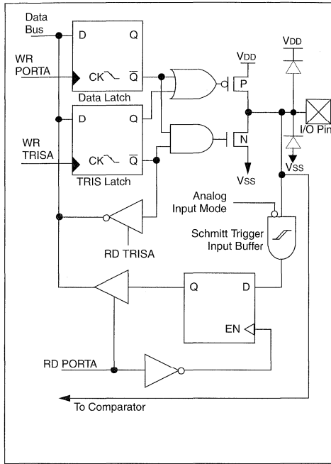
FIGURE 5-1: BLOCK DIAGRAM OF RA0/AN0:RA1/AN1 PINS
