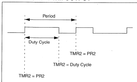
FIGURE 10-4: PWM OUTPUT
