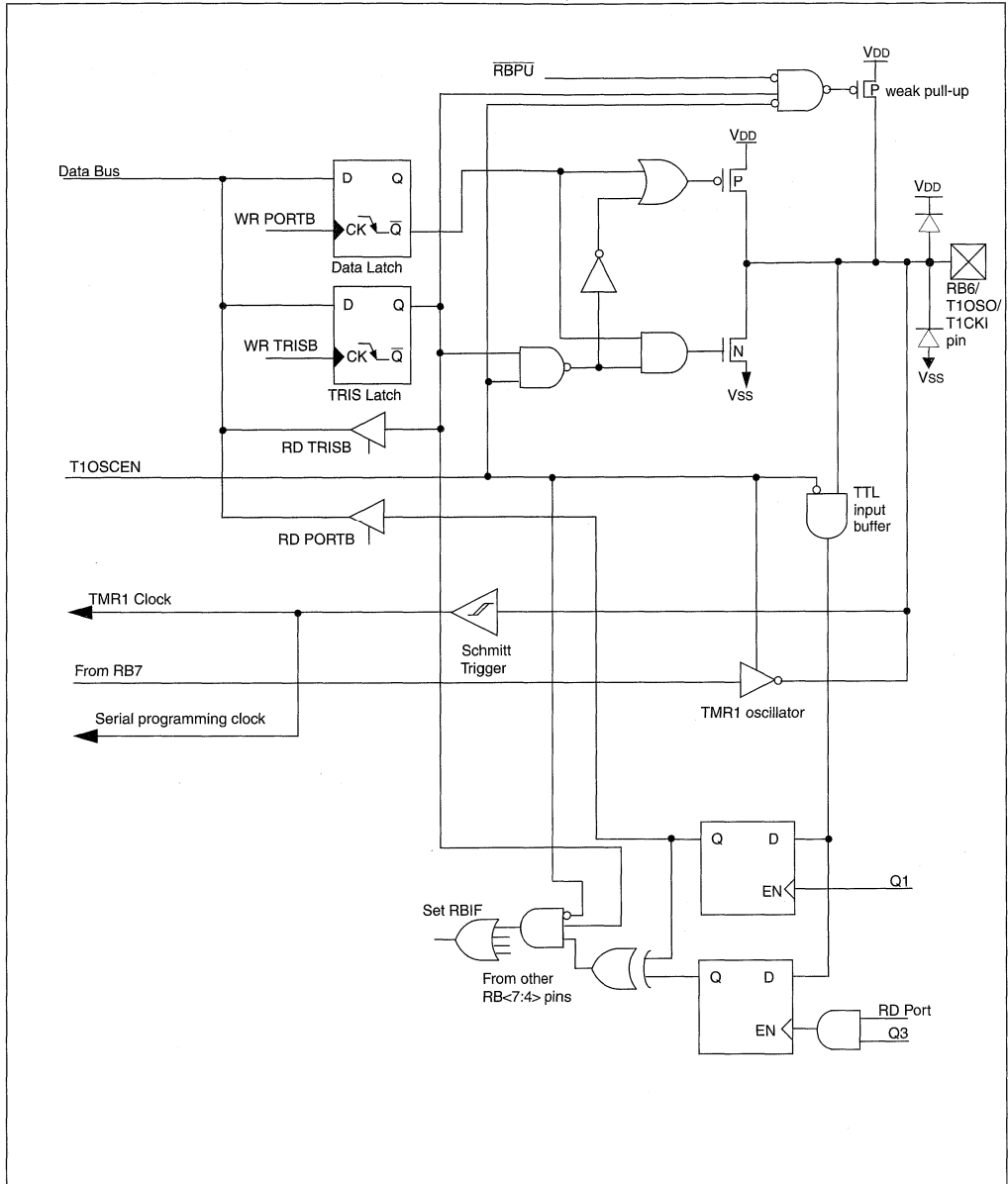
FIGURE 5-14: BLOCK DIAGRAM OF RB6/T1OSO/T1CKI PIN
